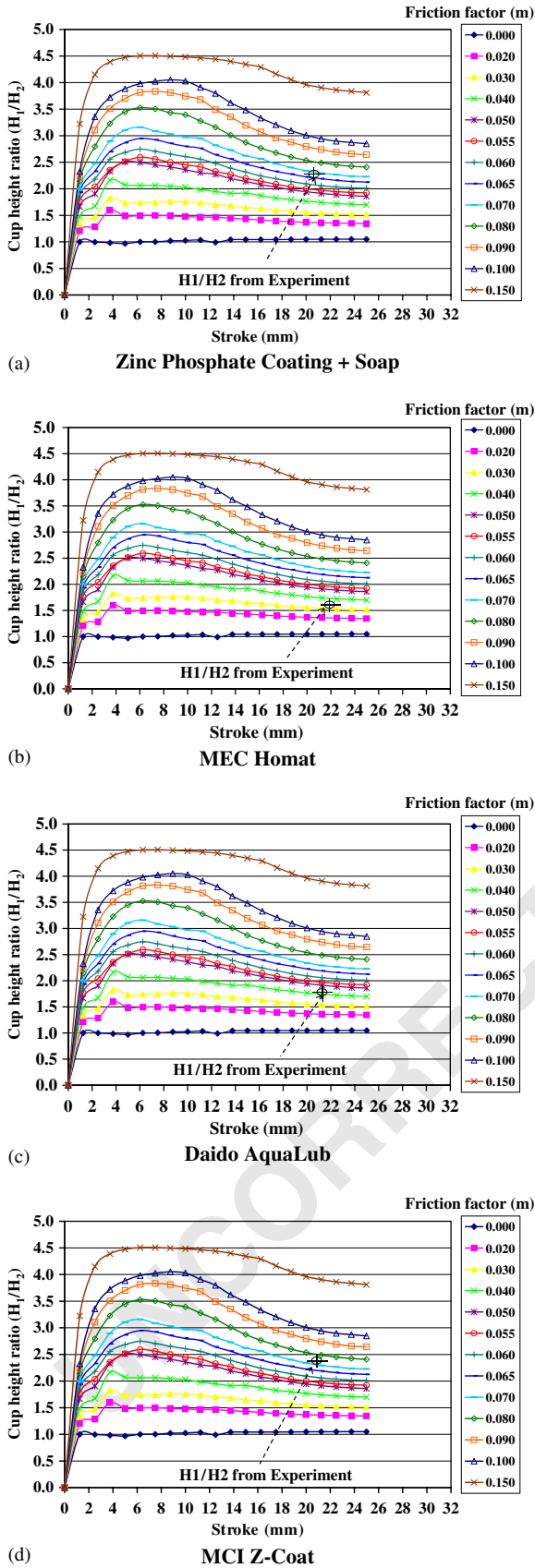
Fig. 13. Determination of friction factors for the four lubricants tested.
