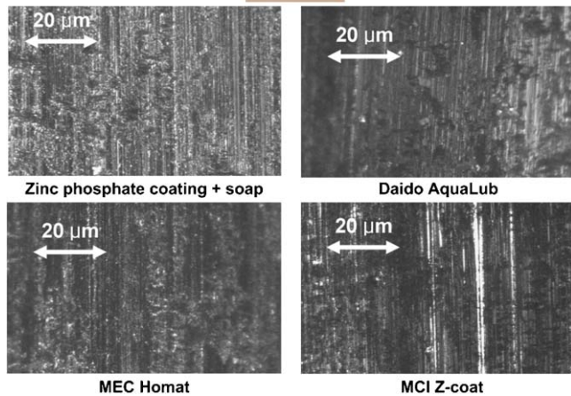
Fig. 16. Optical micrographs of the upper cup after tests.
