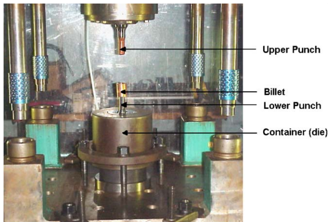
47 Fig. 5. ERC/NSM double cup backward extrusion test tooling.
