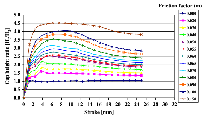
Fig. 9. Friction factor calibration curves.
