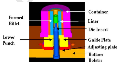
57 Fig. 6. Cross-sectional view of double cup backward extrusion tooling.
